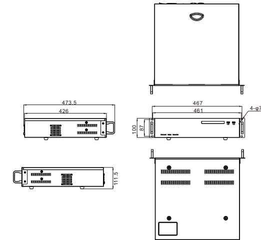
Figure 2-1 Dimensions (Unit:mm)
